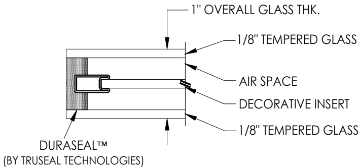
G3 GLAZING DETAIL DECORATIVE
