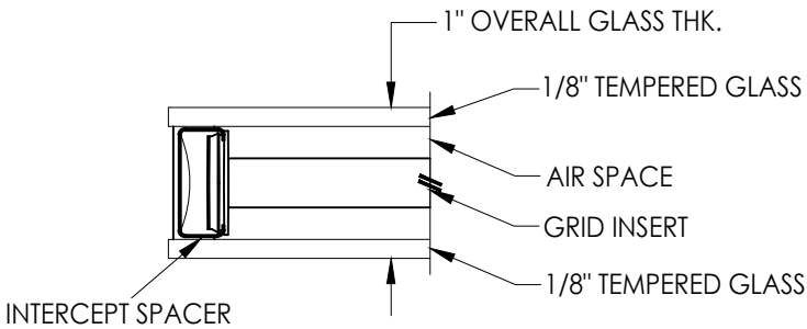
G2 GLAZING DETAIL GRIDS BETWEEN GLASS
