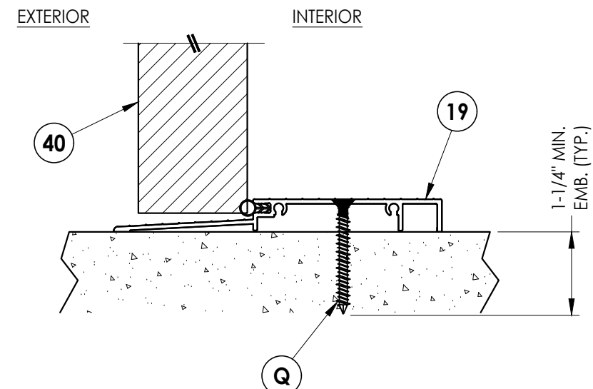
4 7 VERTICAL CROSS SECTION ADA Outswing Sill
