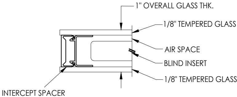
G4 GLAZING DETAIL BLINDS BETWEEN GLASS
